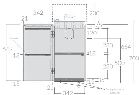
VISTA FRONTALE FRONTAL VIEW
