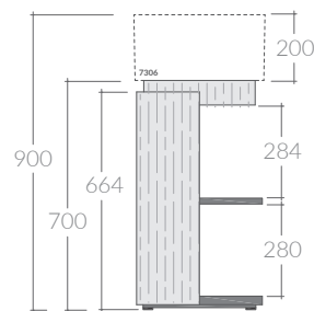
VISTA LATERALE SIDE VIEW
